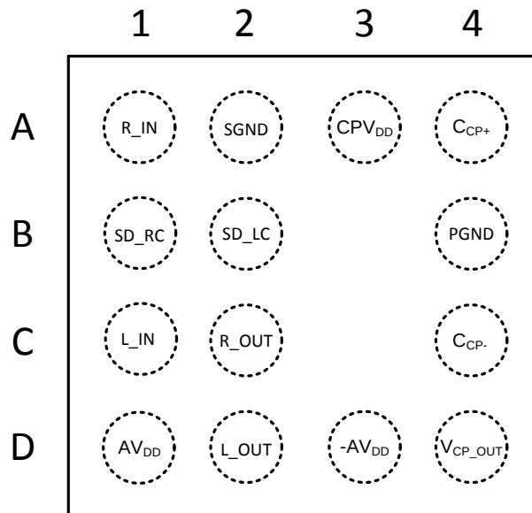
Figure 2. DSBGA Package Top View See Package Number YZE0014
